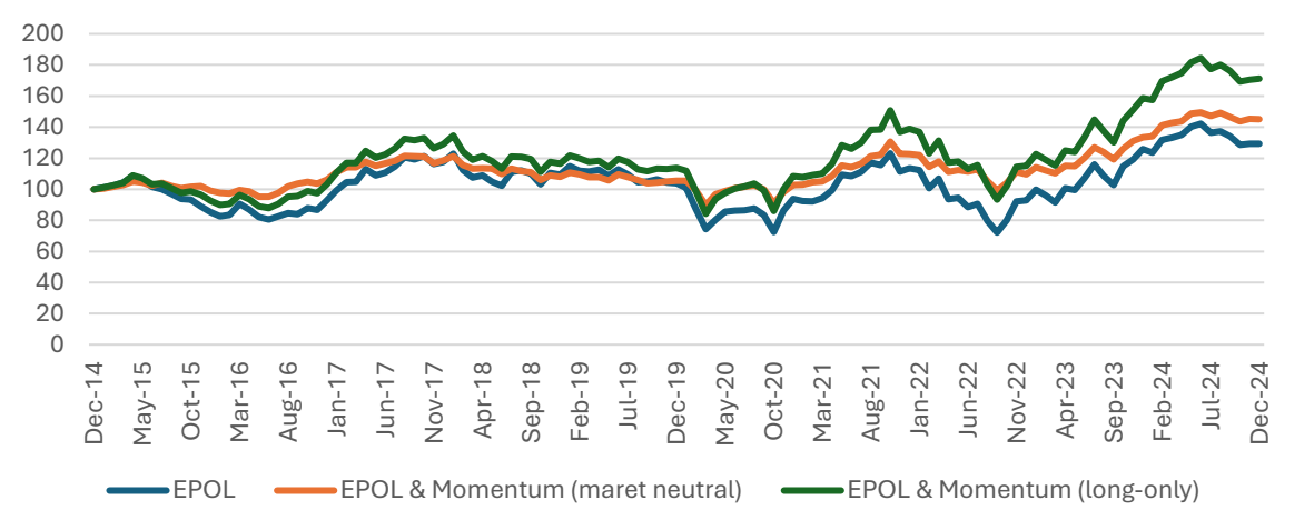
Figure 10. Cumulative net returns to a passive broad market fund against two momentum-based diversification strategies
