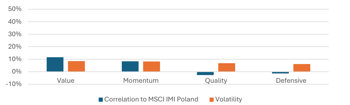
Figure 9. Average in-sample volatility and correlation estimates for market-neutral factor-tilted portfolios (2014-2024)
