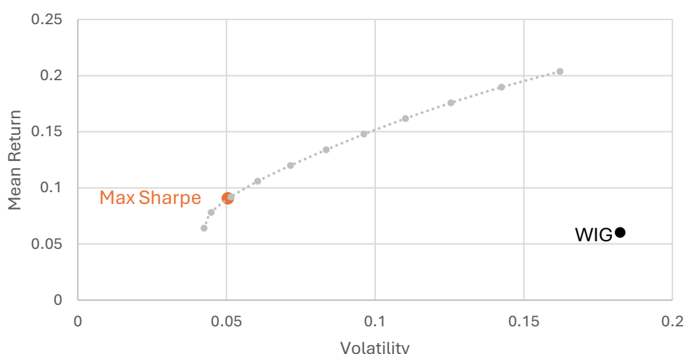
Figure 1. Mean-variance optimization involving Value, Momentum, Quality and Defensive
